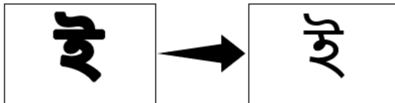
Figure 2.5: Opening operation.
